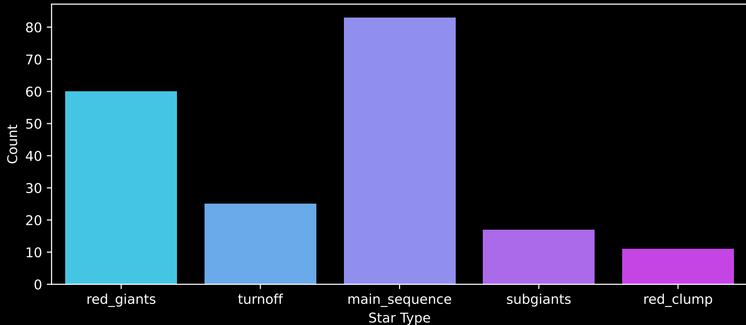
APOGEE DR17 Field: [K2_C7_008-12_btx] Count plot of Star Type
