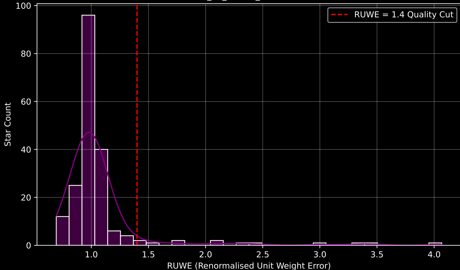
GAPOGEE DR17 Field [K2_C7_008-12_btx] RUWE Distribution (n= 196)
