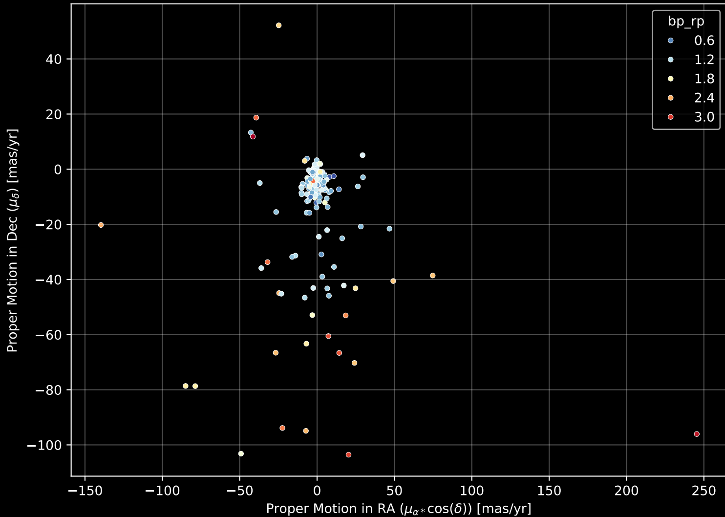
APOGEE DR17 Field: [K2_C7_008-12_btx] Proper Motion Diagram (n= 196)
