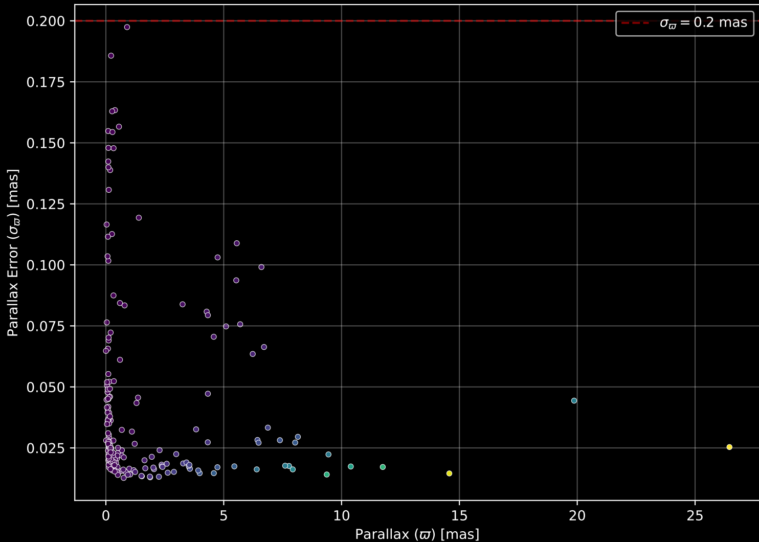
APOGEE DR17 Field: [K2_C7_008-12_btx] Parallax Quality (n= 196)
