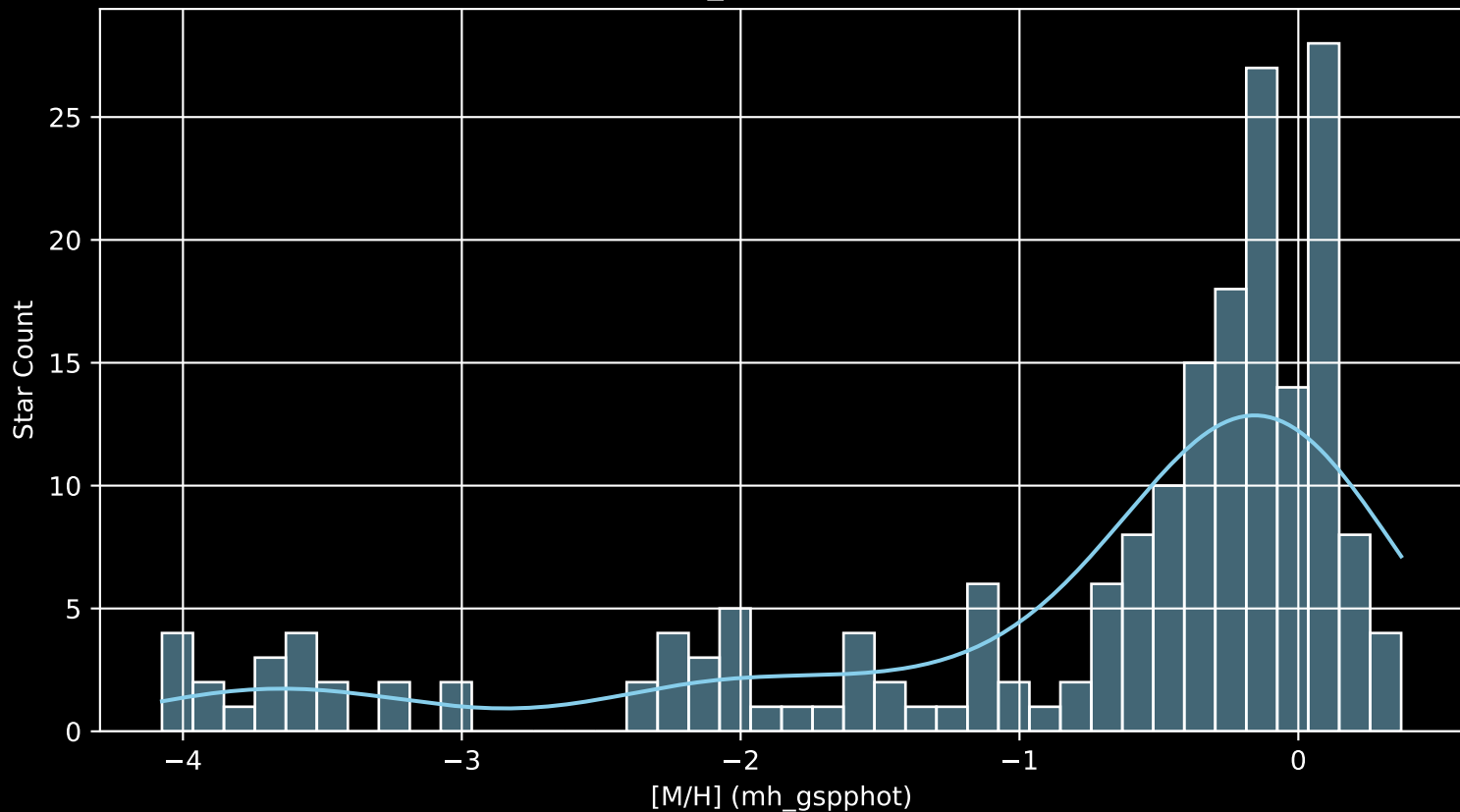
APOGEE DR17 Field: [K2_C7_008-12_btx [M/H] (mh_gspphot) (n= 194)
