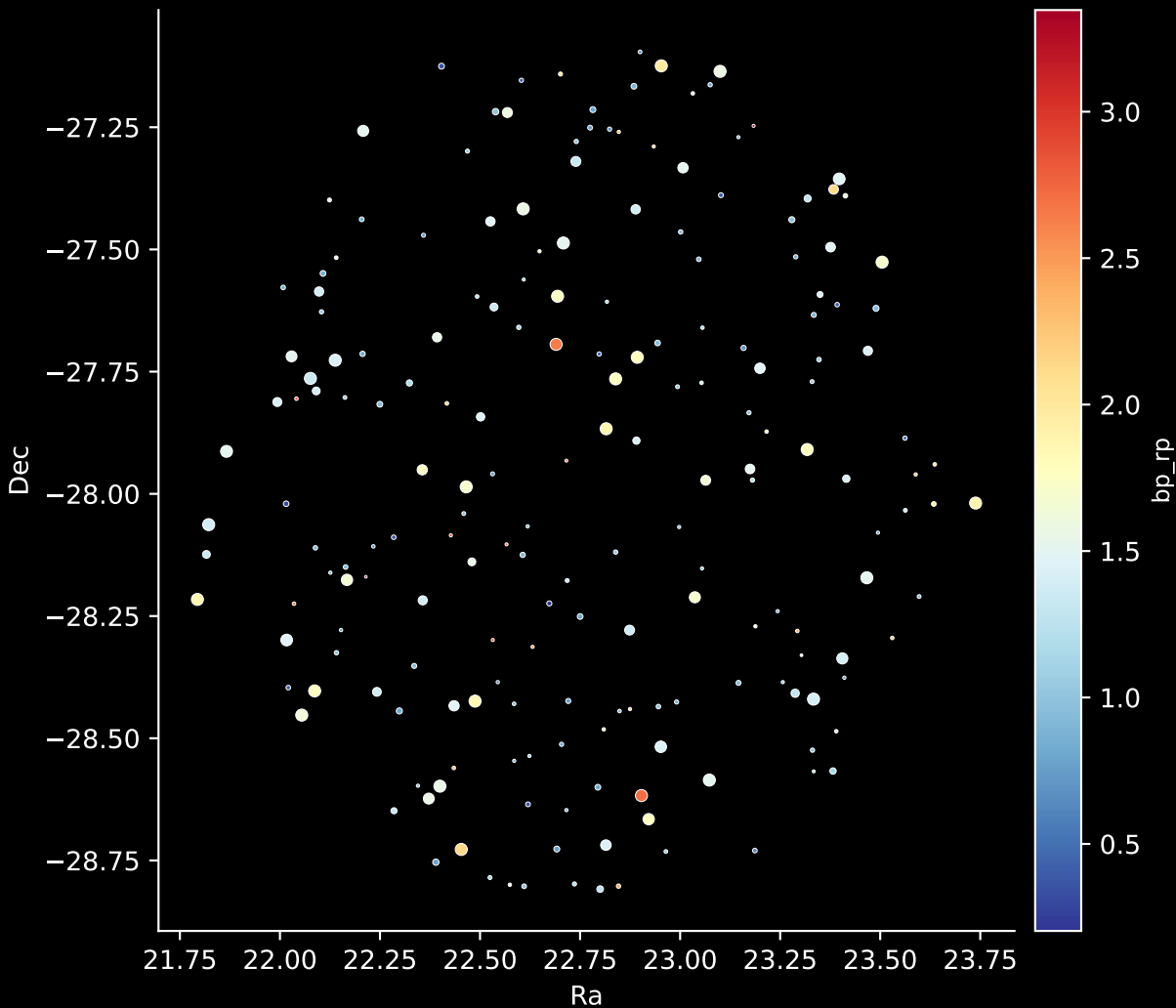
APOGEE DR17 Field: [K2_C7_008-12_btx] Stars: 196
